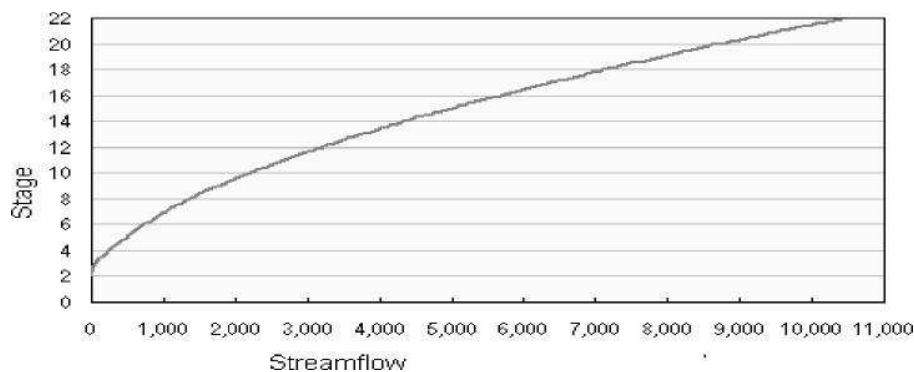
Figure 11.4: Rating curve defines stage/streamflow relation
