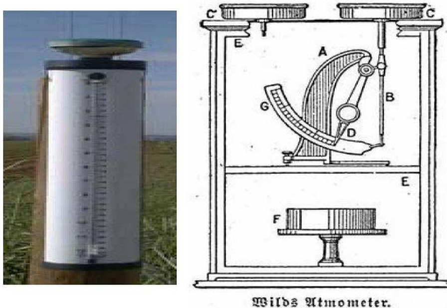
Figure 7.4: Image of an atmometer for obtaining direct measurement of evaporation
