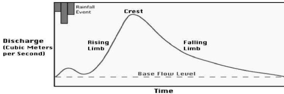
Figure 10.1: Stream hydrograph.
